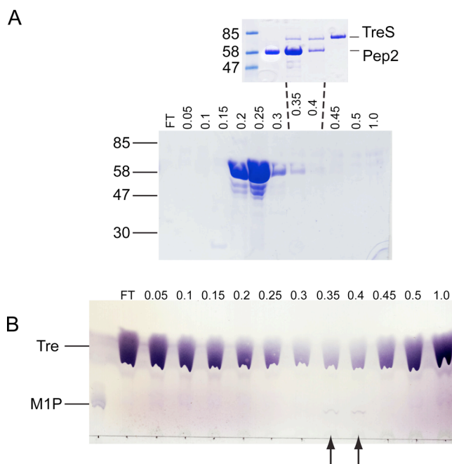
Figure 7. Evidence for formation of the TreS:Pep2 complex in M. smegmatis mc 2 155. (A) His 6 -tagged Pep2 was purified from M. smegmatis extracts by Ni-NTA and ion exchange chromatography, and anion exchange column fractions were analyzed by Coomassie-stained SDS-PAGE, with NaCl concentrations (in M, across the top), and molecular weight standards (in kDa, on the left) as indicated. FT = flow through. (A, inset) Coomassie-stained SDS-PAGE of ion exchange fractions eluted at 0.35 and 0.4 M NaCl after ~20-fold concentration, flanked by TreS- and Pep2 controls. (B) Thin-layer chromatogram of reactions mixtures (100 μL) containing 100 mM trehalose (Tre) and 20 μL of fractions of the anion exchange column fractions shown in panel A. The position of maltose-1-phosphate (M1P) and NaCl concentrations (in M) are indicated. Arrows highlight the two fractions producing maltose-1-phosphate.
